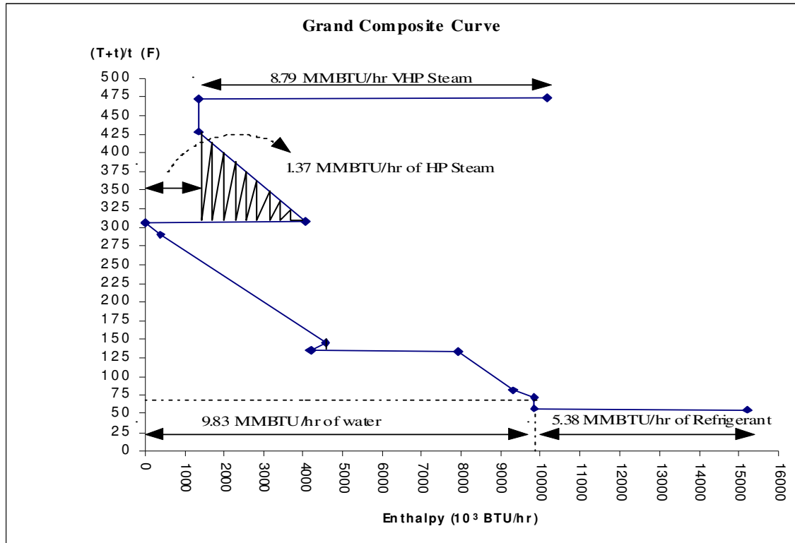
Figure 6.6 Grand Composite Curve for Scenario (4)
