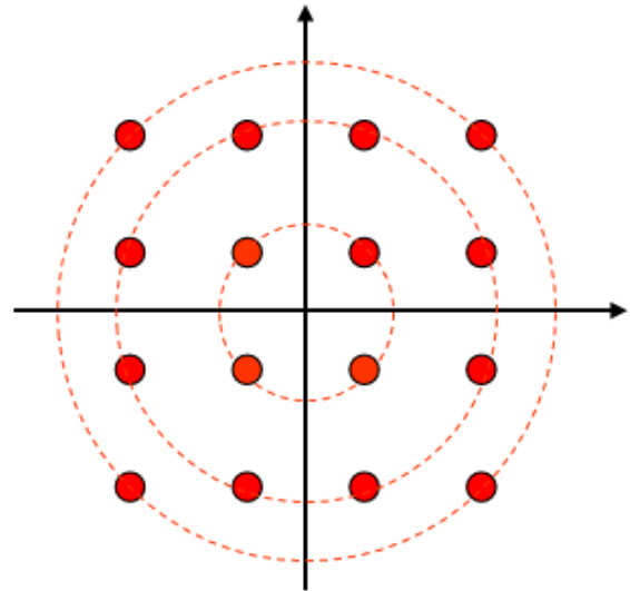
16 QAM
