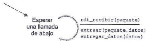
b. rdt1.0: lado receptor
