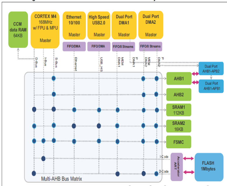
Figure 7. STM32F405/415 and STM32F407/417 system architecture
