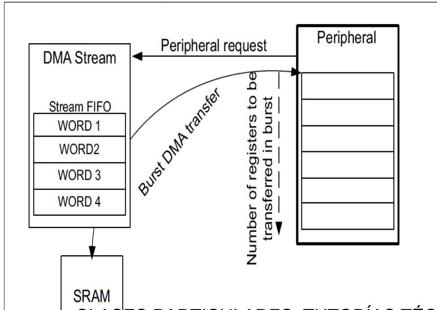
Figure 5. DMA burst transfer
