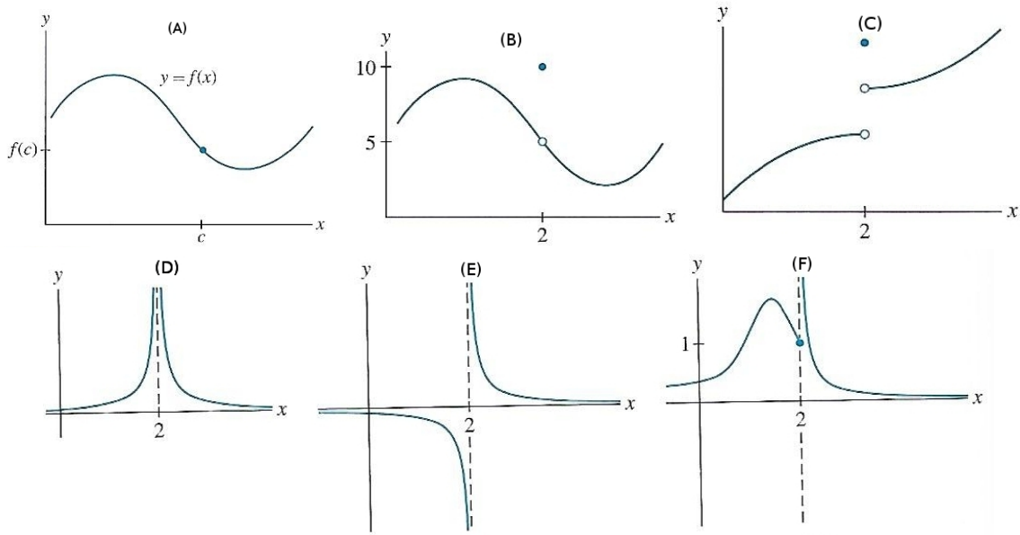
Figure 1: Graphs of a continuous function (A), an evitable discontinuity (B), a jump discontinuity (C) and several cases of essential discontinuity (D-F), from p. 62 (A), 63 (B,C) and 64 (D-F) of [1].
