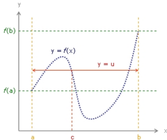
Figure 2: Illustration of the intermediate value theorem. Source: [2].
