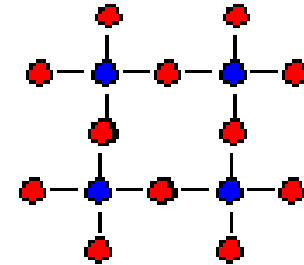
Covalent solid
