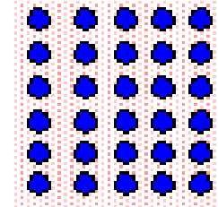
Metallic solid
