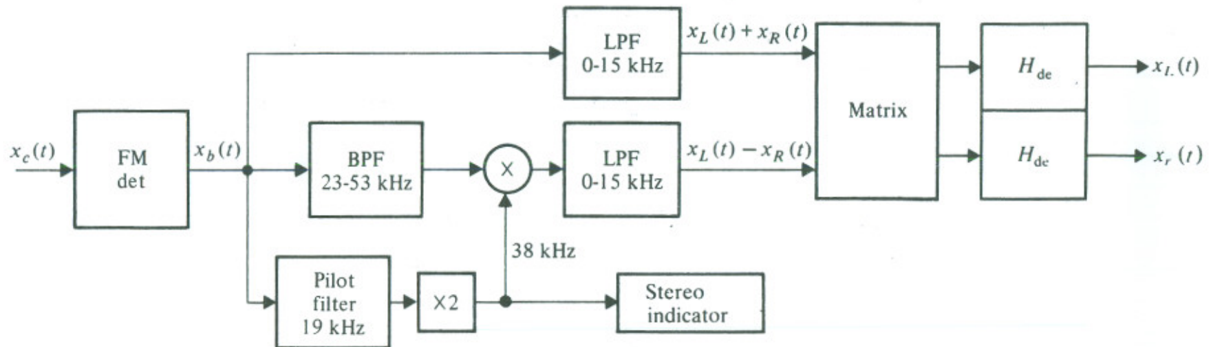
Figure 8.2-6 FM stereo multiplex receiver.
