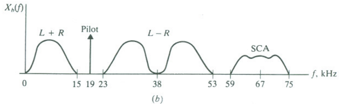
Figure 8.2-5 FM stereo multiplexing. (a) Transmitter; (b) baseband spectrum.
