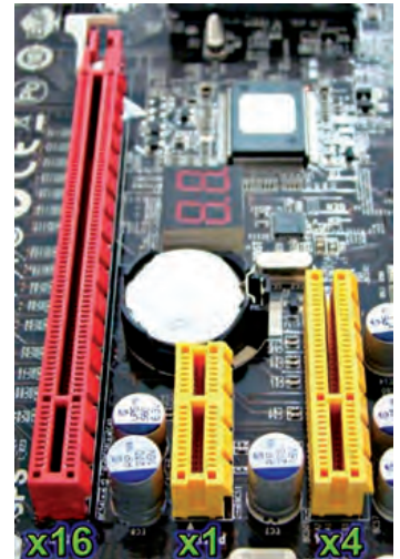
↑ Slots PCI-Express.
