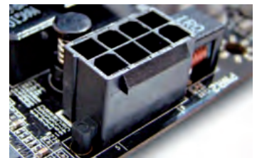
↑ Conector de corriente EATX12 V.
