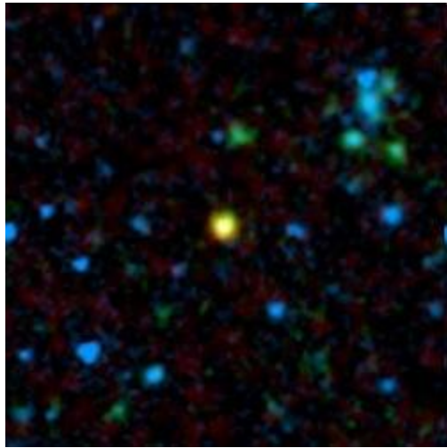
This false-color image from NASA's Spitzer Space Telescope shows a distant galaxy (yellow) that houses a quasar , a super-massive black hole
