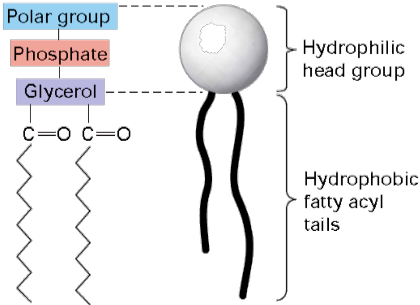
Glycerophospholipid
