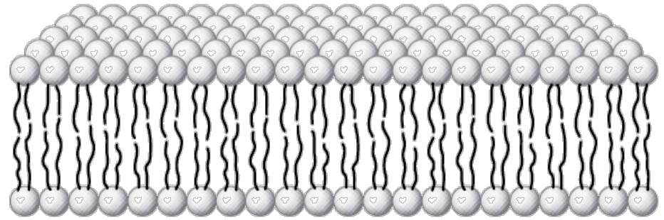
Phospholipid bilayer
