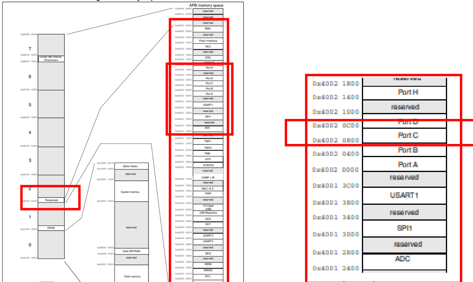
Figure 9. Memory map
