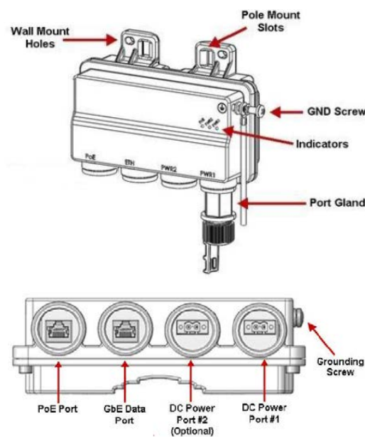
FIGURA 12.14: PoE CERAGON.
