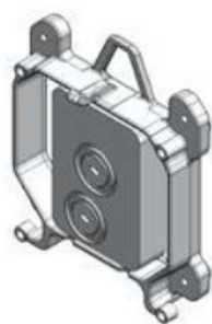
FIGURA 12.12: SPLITTER DUAL PARA ODU FULL-OUTDOOR DUAL-CORE IP20-C.
