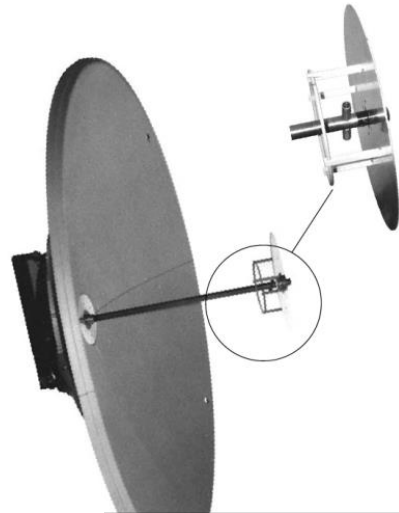
Spiral wire antenna on corrugated disk
