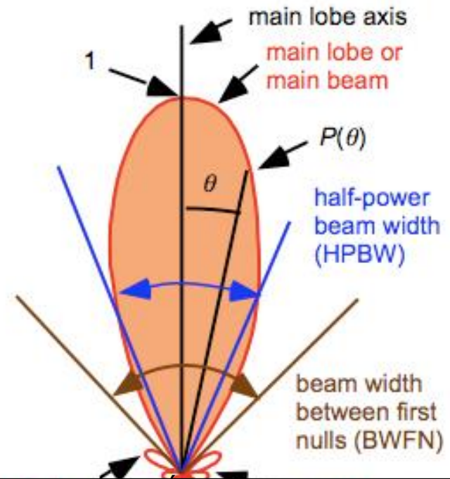
Power pattern
