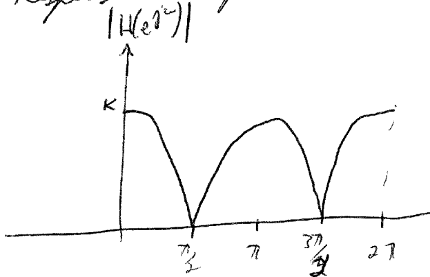
H_2(z)
