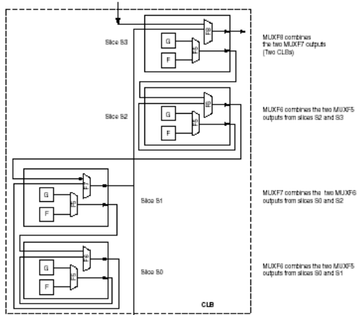
Figure 22: MUXF5 and MUXF6 multiplexers
